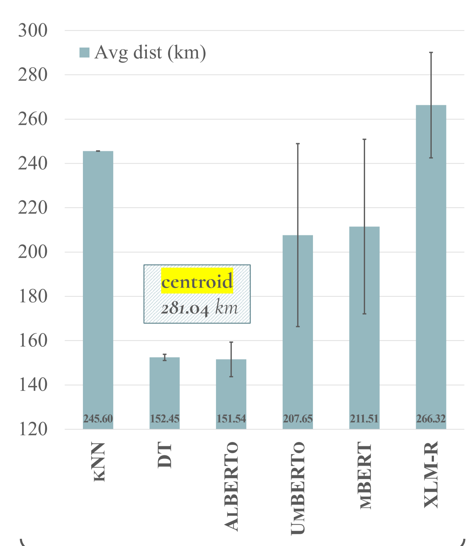
FINE-GRAINED GEOLOCATION
