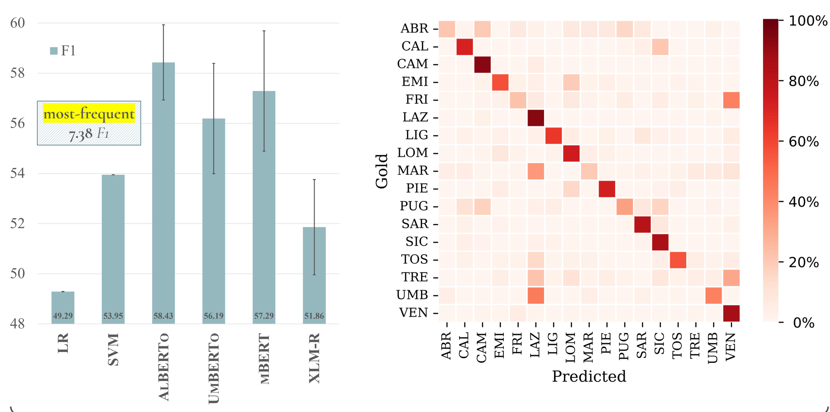
COARSE-GRAINED GEOLOCATION
